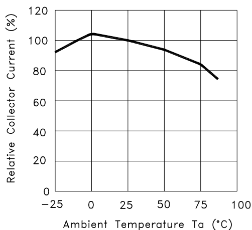
Fig.4 Collector Current I C vs. Ambient Temperature
